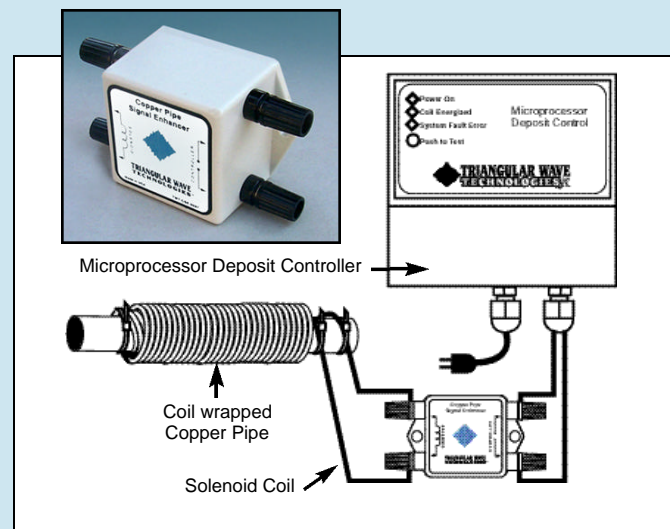
Schematic rendering of the TWT-CSE-0227 hookup
