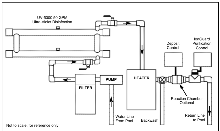
Typical installation overview of pool/spa equipment room. TWT products (sizes) will vary according to pool size and volume of water. See sections B3 and B5 of TWT catalog for additional information.
