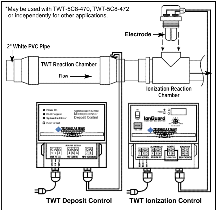
TWT Deposit Control/Ionization Purification System 2-inch Ionization Unit with Integrated* TWT-5C8-402
